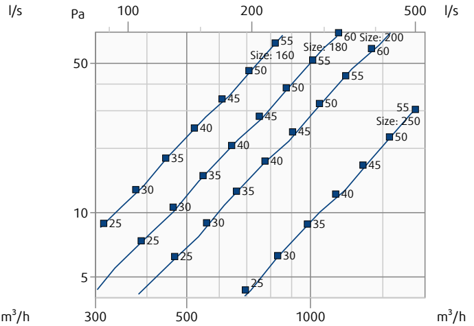
Pressure drop & A-weighted sound power level in dB(A)
