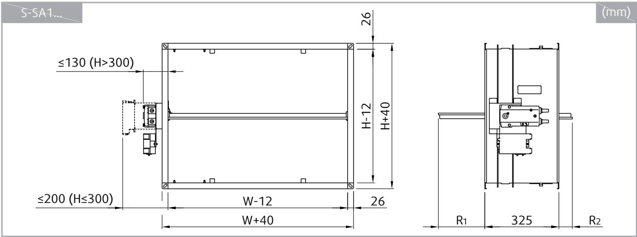
Dimensions of S-SA1
