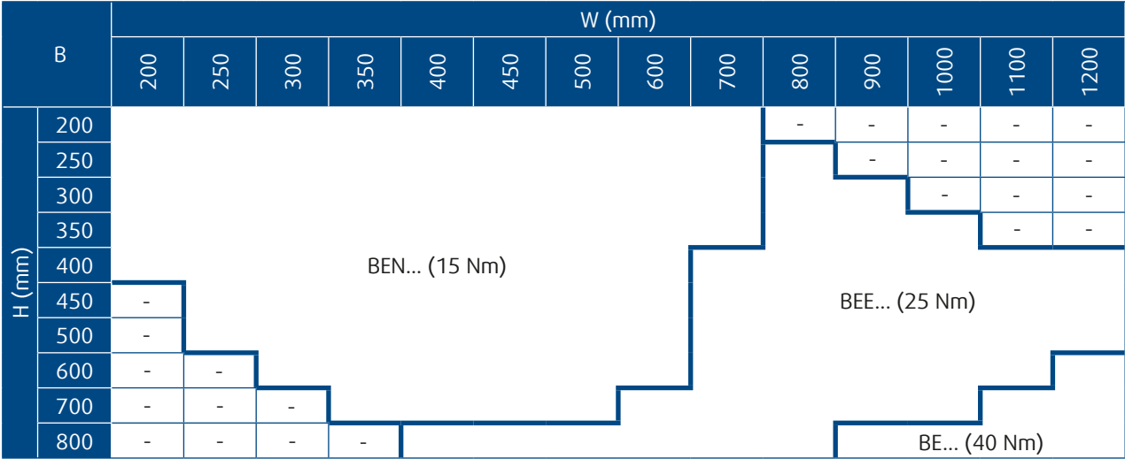
Actuator Size Map of S-SA1
