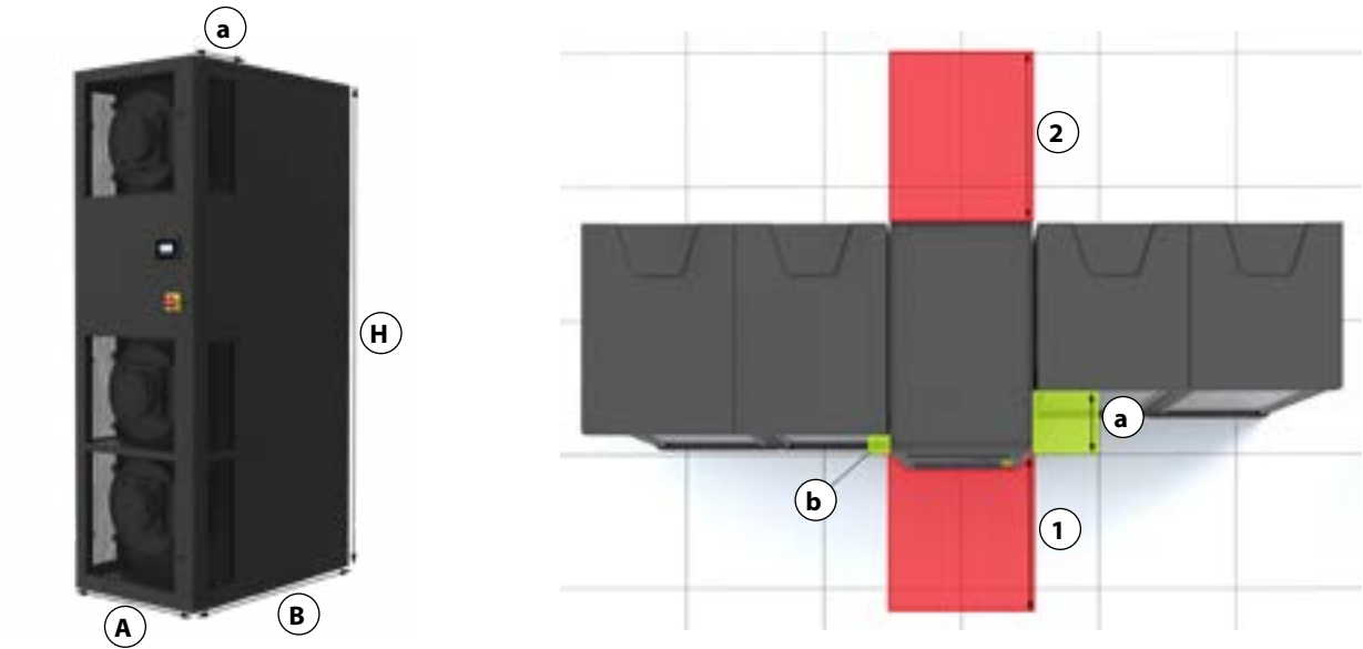
Series R clearance spaces
