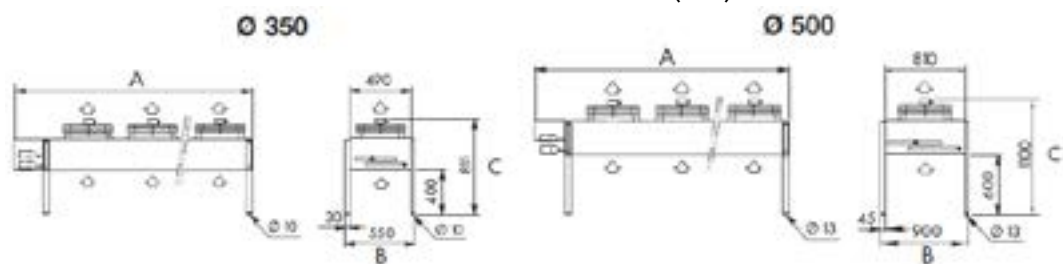
Horizontal Installation ( H )
