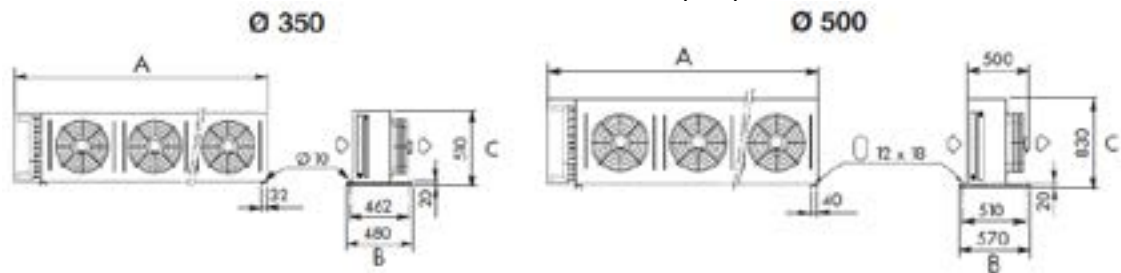
Vertical Installation ( V )
