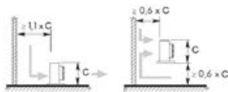
Vertical Installation ( V )
