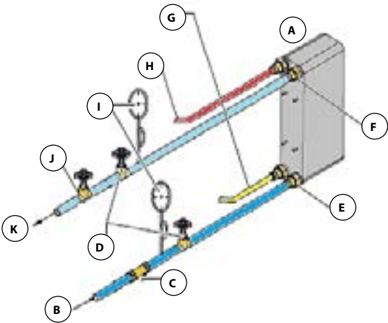
Water connections
