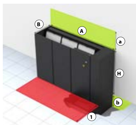
Series G clearance spaces
