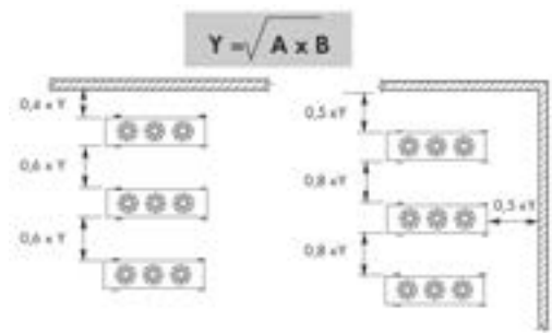
Horizontal Installation ( H )
