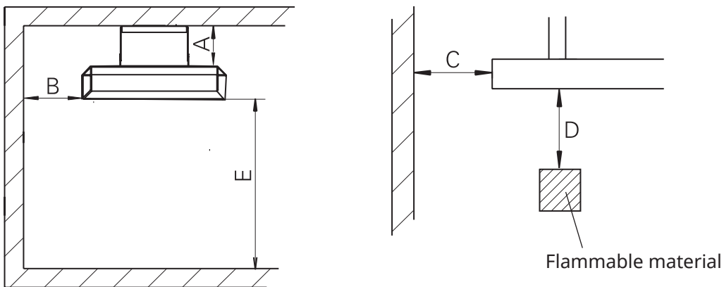
Fig.3. Minimum distances
