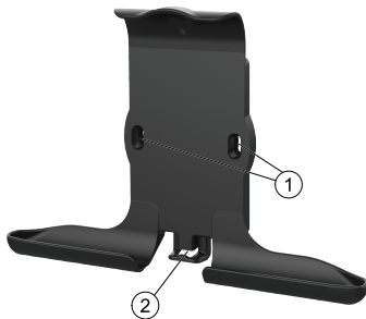
Fig. 2 Holder for NaviPad, (1) fixing points, (2) cable hook
