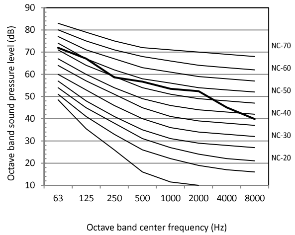
Figure 2-10.7: 18HP octave band level
