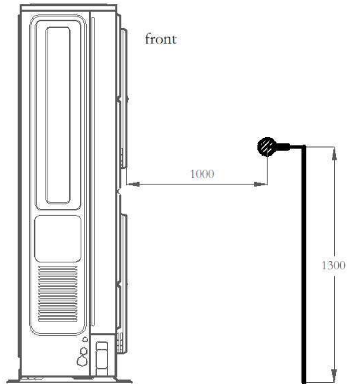
Figure 2-10.1: Sound pressure level measurement (unit: mm)
