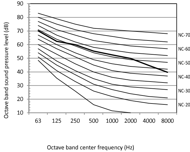
Figure 2-10.2: 8HP octave band level
