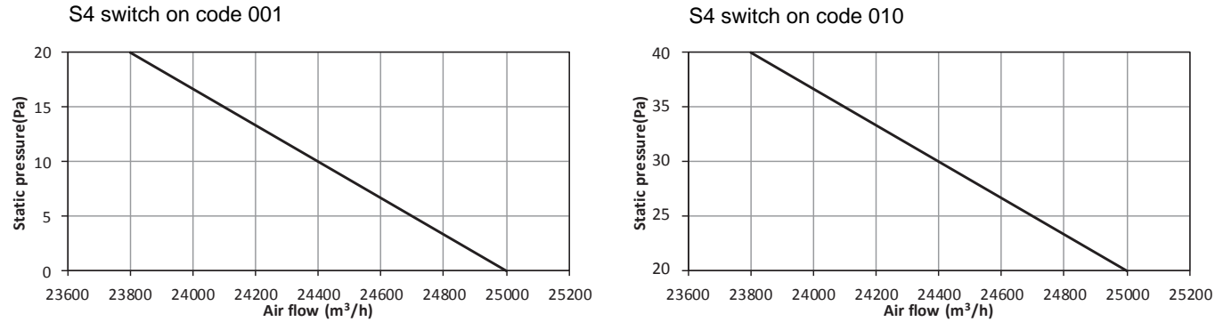
Fig. 4-28: 24-28HP units fan performance
