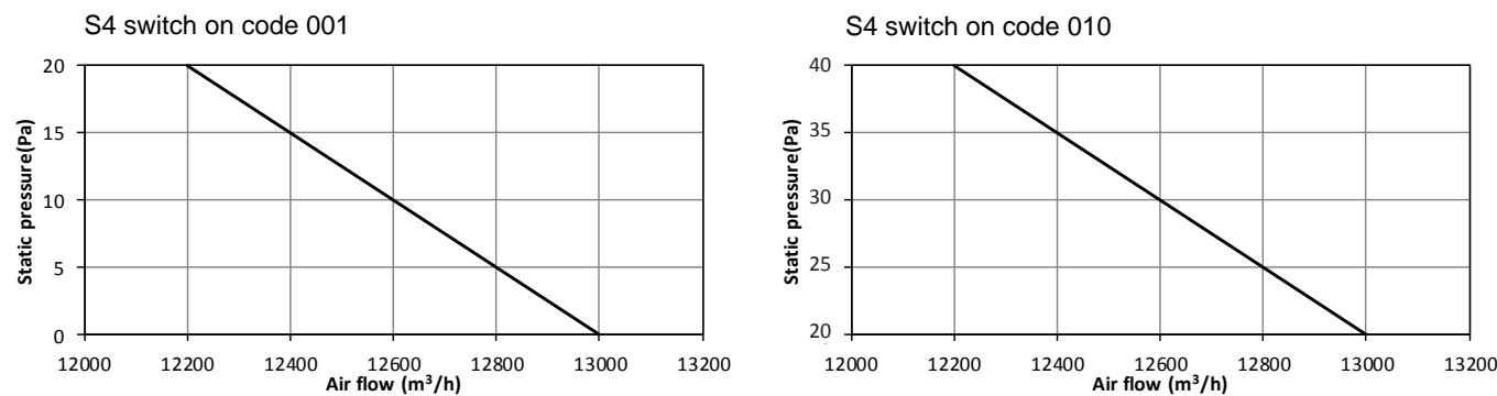
Fig. 6: 14-16HP units fan performance
