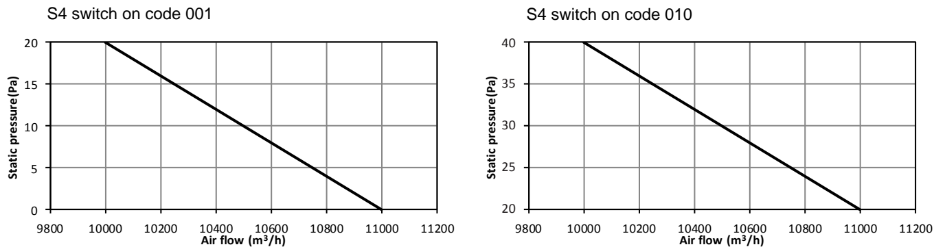
Fig. 4-25: 8-12HP units fan performance
