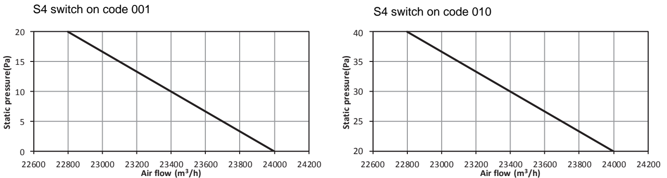
Fig. 4-29: 30-32HP units fan performance
