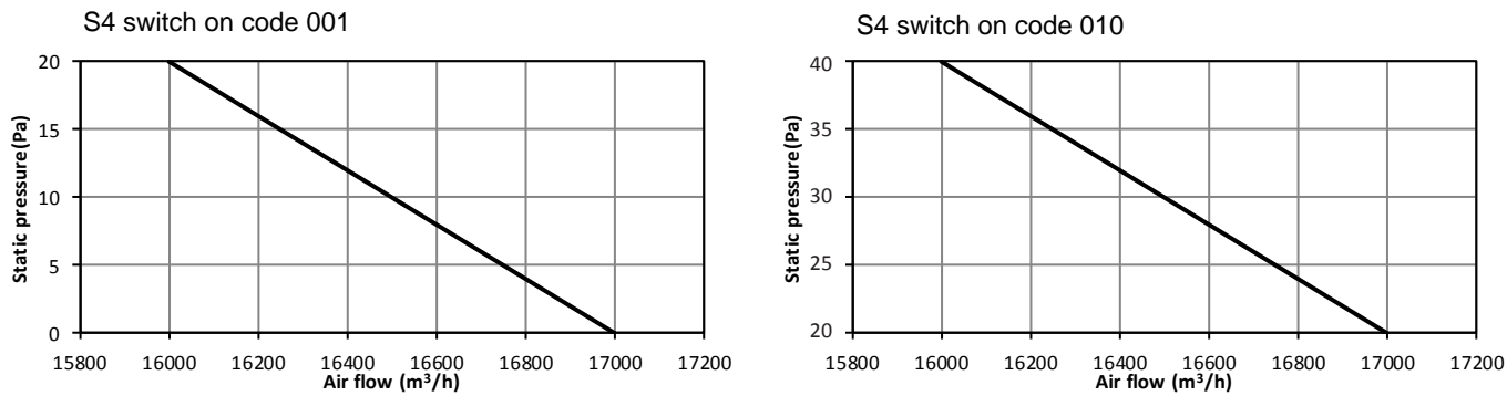
Fig. 4-27: 18-22HP units fan performance
